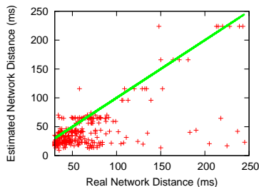
Figure 1: Targeted close node attack results on GNP
