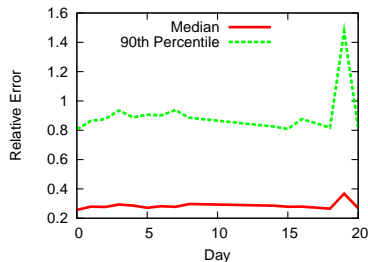
Figure 4: Median and 90th percentile relative error using 12/01/09 positions for estimation measurements through 12/21/09, by day.
